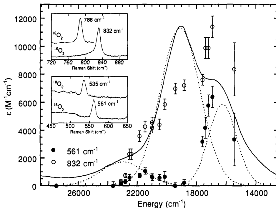
Figure 8. Absorption spectrum of the trans end-on dimer [\{\text{Cu}(\text{TMPA})_2(\text{O}_2)\}_2]^{2+} with resonance Raman profiles for the O-O and Cu-O peaks. The O-O and Cu-O Raman peaks for ^{16}\text{O}_2 and ^{18}\text{O}_2 isotopes of the complex are shown in the insets.
