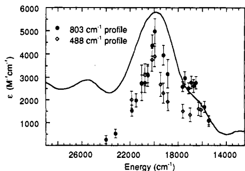
Figure 5. Charge-transfer absorption spectrum of the end-on monomer [\text{Cu}_2(\text{XYL-O})(\text{O}_2)]^+ with resonance Raman excitation profiles for the O-O stretch ( 803\text{ cm}^{-1} ) and the Cu-O stretch ( 488\text{ cm}^{-1} ).
