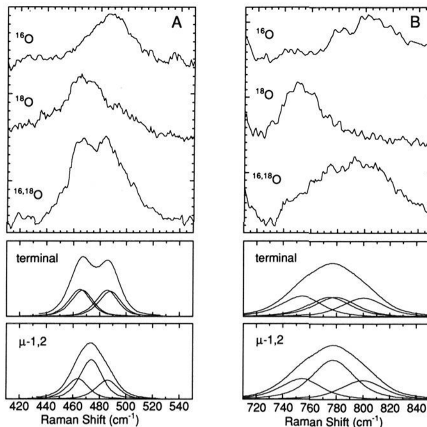
Figure 4. Resonance Raman spectra of the end-on monomer [Cu_2(XYL-O-)(O_2)]^+ showing (A) the Cu-O stretch and (B) the O-O stretch for ^{16}O_2 , ^{16}O^{18}O , and ^{18}O_2 isotopes. Below these are simulated spectra based on the experimental frequencies and line shapes of these peaks assuming either a symmetric ( \mu -1,2) or asymmetric (terminal) binding geometry.
