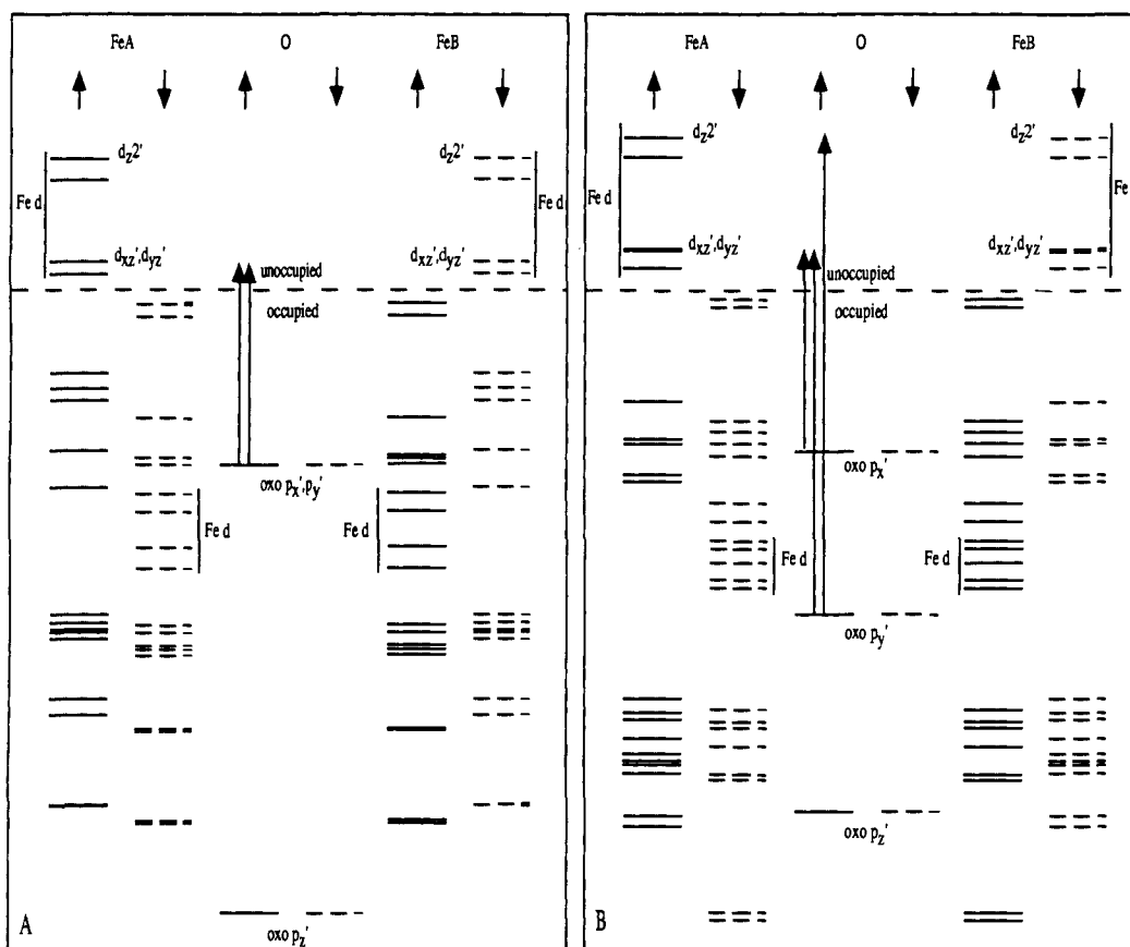
Figure 36. Energy level diagrams from BS-SCF-X \alpha -SW calculation on (A) a linear monobridged and (B) a tribridged (Fe-O-Fe angle = 120 ^\circ ) complexes.
