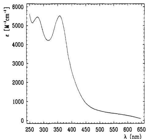
Figure 25. Spectra of doubly bridged cis - \mu -1,2- \text{O}_2^{2-} binuclear \text{Co(III)} systems.
