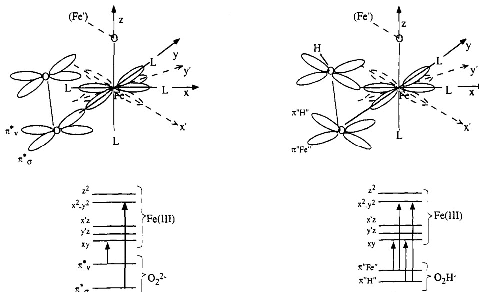
Figure 39. Qualitative bonding description of \text{O}_2^{2-}\text{-Fe(III)} (left) and \text{HO}_2\text{-Fe(III)} (right). Note that for \text{O}_2^{2-} only two transitions are predicted, one more intense than the other, while for \text{HO}_2^- there should be four of equal intensity.
