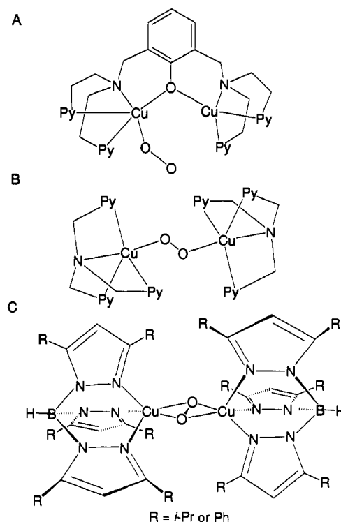
Figure 2. Peroxo-copper complexes with different peroxide binding geometries: (A) end-on monomer, [Cu 2 (XYL-O-)(O 2 )] + , (B) trans end-on dimer, [ \{Cu(TMPA)\}_2(O_2)\}^{2+} , and (C) side-on dimer, [Cu(HB(3,5- i -Pr 2 p z ) 3 )] 2 (O 2 ).
