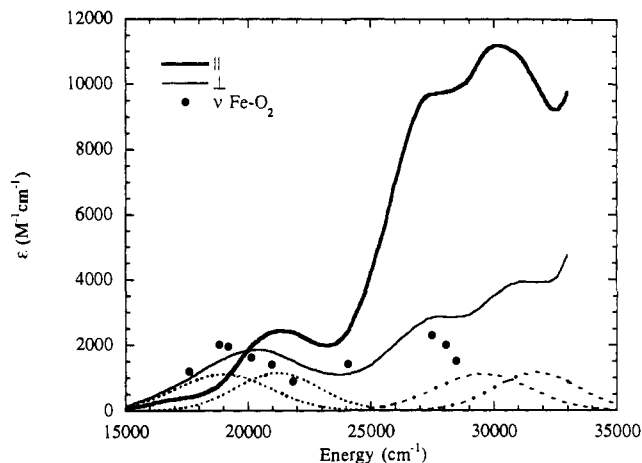
Figure 38. Polarized single-crystal absorption spectra for oxyHr and the Fe-O 2 rR profile. Dashed lines are a fit giving four O 2 2- → Fe(III) transitions. Points indicate rR excitation profile.
