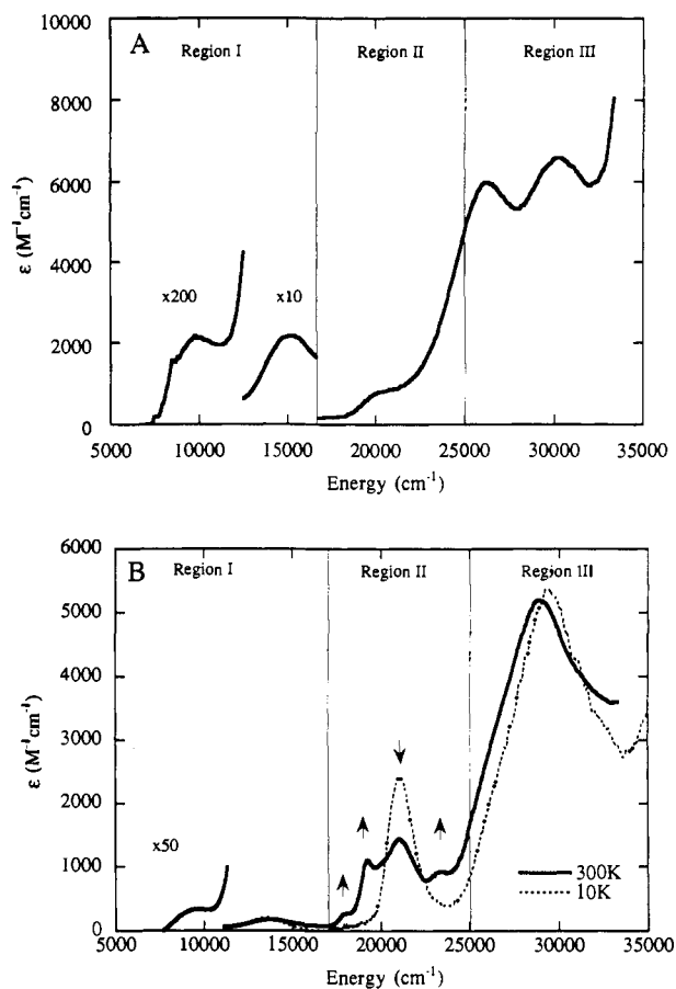
Figure 26. (A) Room-temperature absorption spectrum of metCl- Hr and (B) room-temperature and low-temperature (10 K) absorption spectra of the tribridged model complex.
